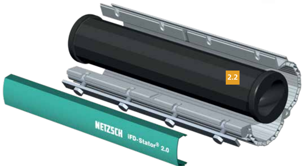
Optional: iFD-Stator® 2.0 Available for sizes NM021 to NM090 in 01L and 02S geometries. Patented design.
