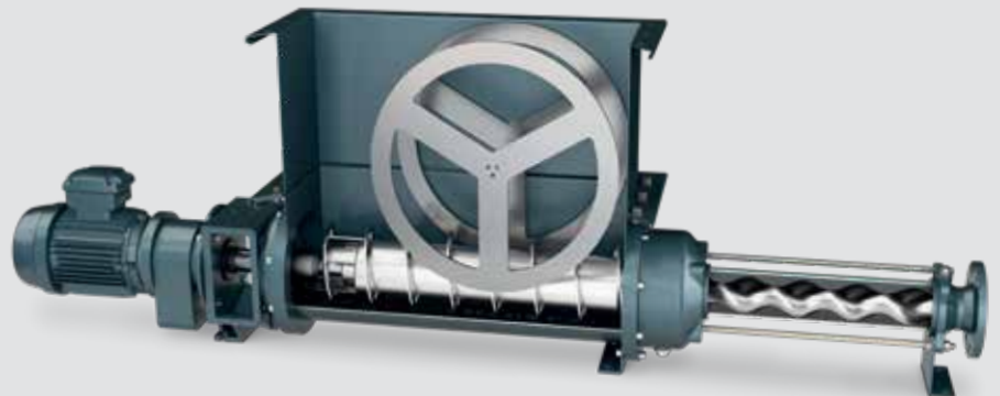
NEMO® Sludge Cake Progressing Cavity Pump with aBP-Module®
