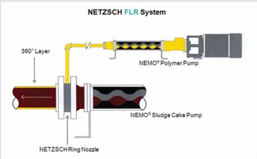
NETZSCH Friction Loss Reduction system
